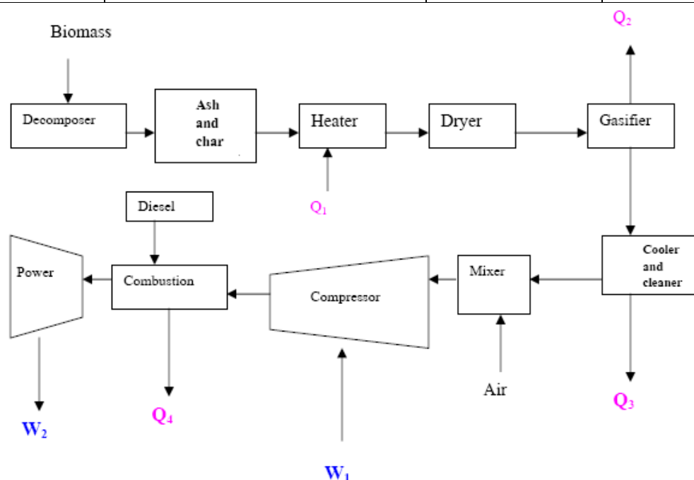
Figure 7: Advanced biomass power with diesel engine (Omer, 2006).
