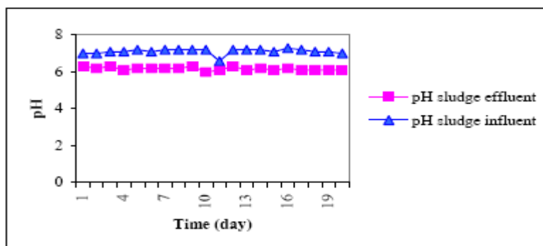
Figure 6: pH sludge before and after treatment in the digester (Omer, 2006).
