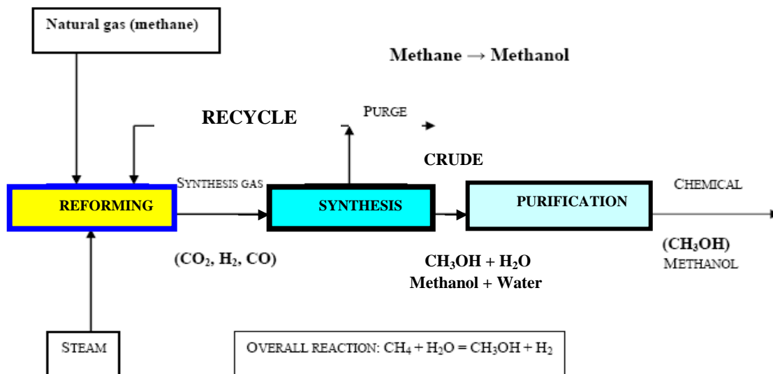
Figure 2: Schematic diagram shows methanol production (Omer, 2006).
